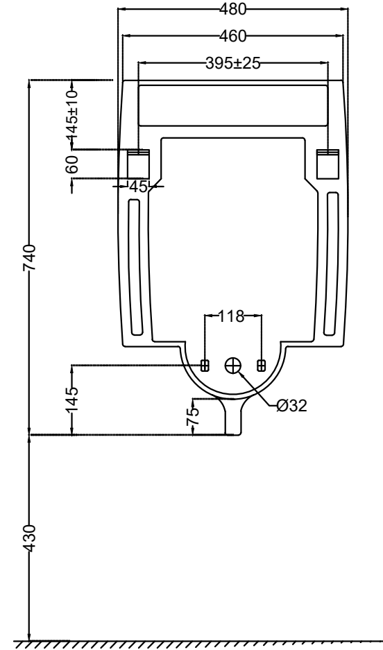
BACK VIEW
