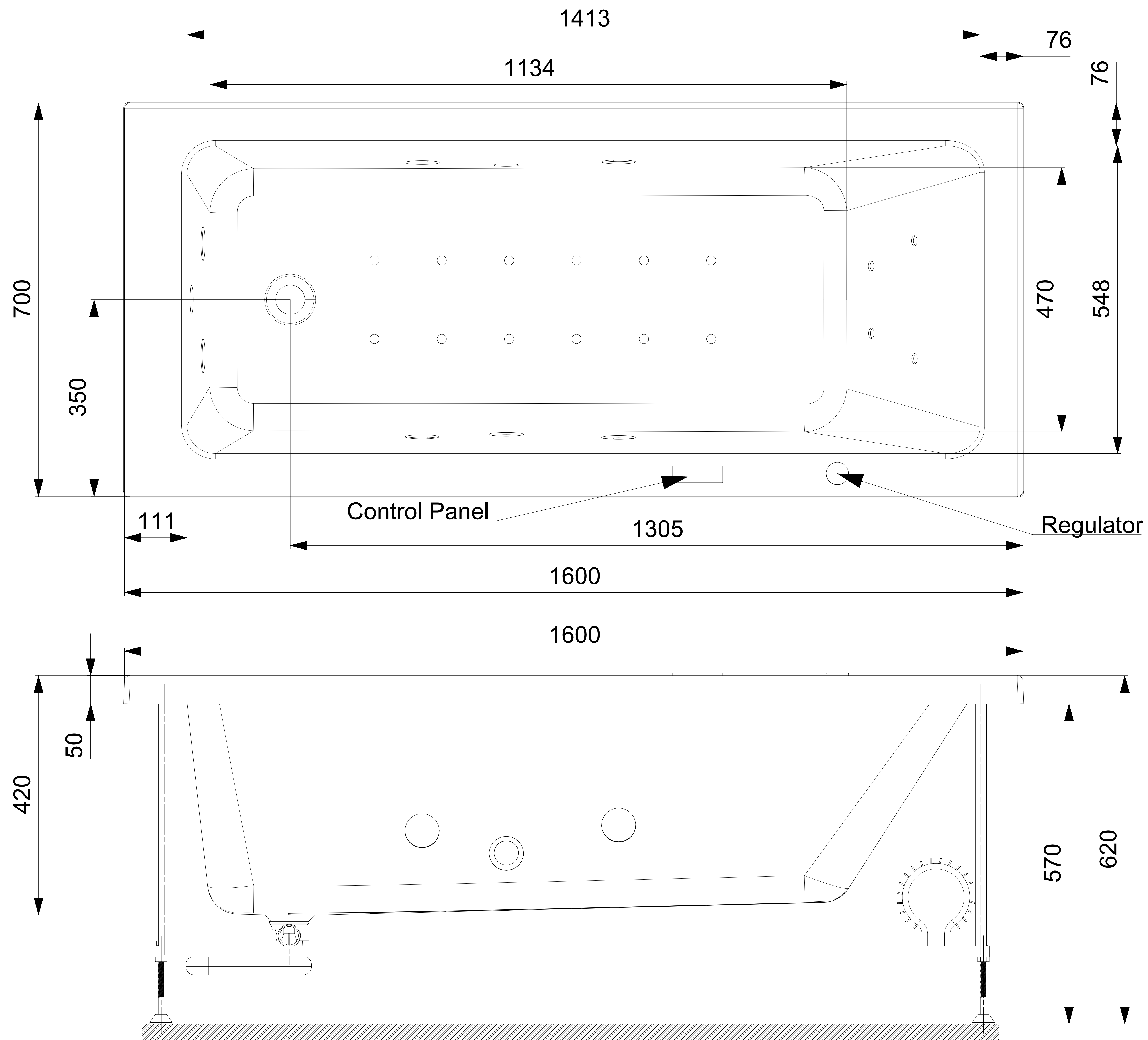
JWP-WHT-FONTE160CX = FONTE 1600X70X420 WHIRLPOOL AND AIRPOOL COMBI SYSTEM
