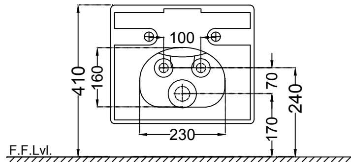
BACK VIEW A
