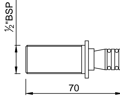
SPOUT NIPPLE
