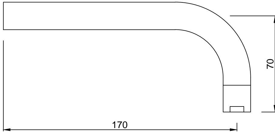
SPOUT
