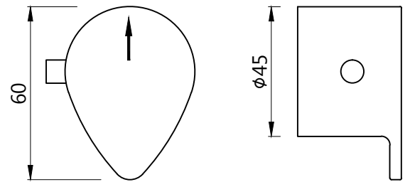
THERMOSTATE HANDLE
