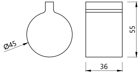
DIVERTER HANDLE
