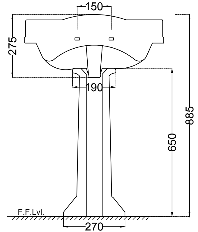
BACK VIEW
