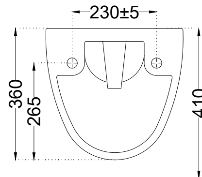
BACK VIEW
