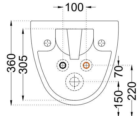
BACK VIEW A
